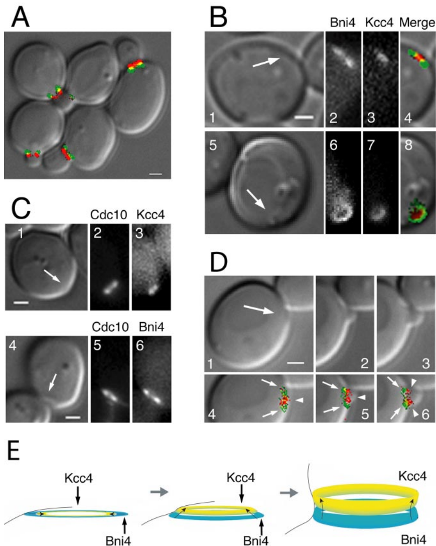
Figure 1. Bni4 and Kcc4 do not colocalize in unbudded cells. DIC and fluorescence images are shown. For merged images, Bni4-CFP and Kcc4-YFP are pseudocolored green and red, respectively. (A) Asymmetric localization of Bni4-CFP and Kcc4-YFP in small- and medium-budded cells of strain YLK189. (B) Spatial separation of Bni4-CFP and Kcc4-YFP in unbudded cells of strain YLK189. (C) Localization of Kcc4-CFP and Bni4-CFP to the inner and outer edges of the Cdc10-YFP septin ring, respectively. 1–3, strain YLK214; 4–6, strain YLK215. (D) Separation of Kcc4-YFP (arrowheads) and Bni4-CFP (arrows) during bud emergence. A cell of strain YLK189 was imaged before bud emergence (1 and 4) and 10 (2 and 5) and 20 (3 and 6) min later. (E) Model showing the location of Bni4 and Kcc4 during the transition of the septin ring into the septin collar upon bud emergence. Bni4 (blue) forms a larger ring that encircles the Kcc4 ring (yellow). At bud emergence, Kcc4 moves toward the growing bud, whereas Bni4 stays on the mother side of the neck. Bars, 1 \mu m.
